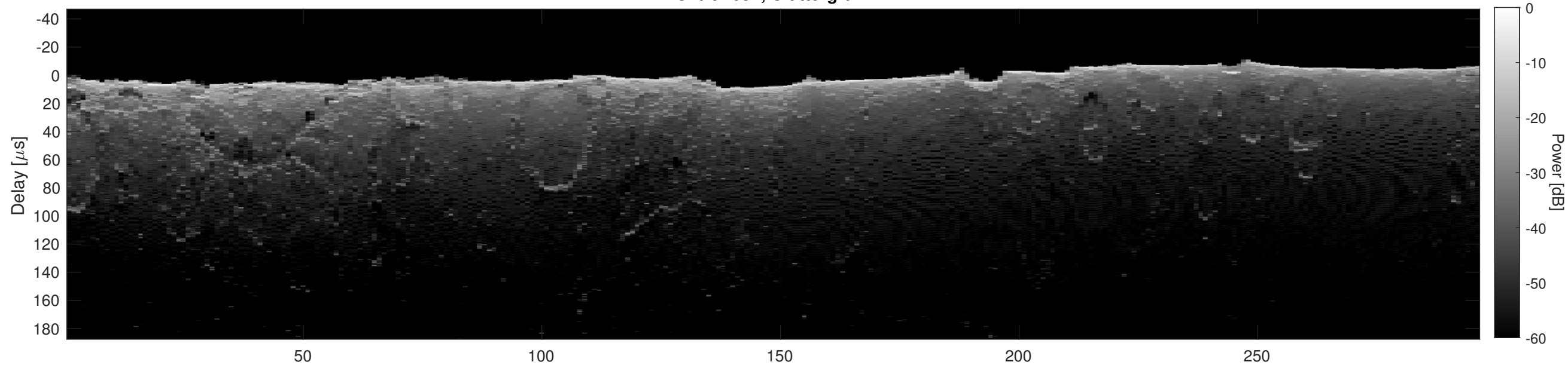
Orbit 2654, Cluttergram
