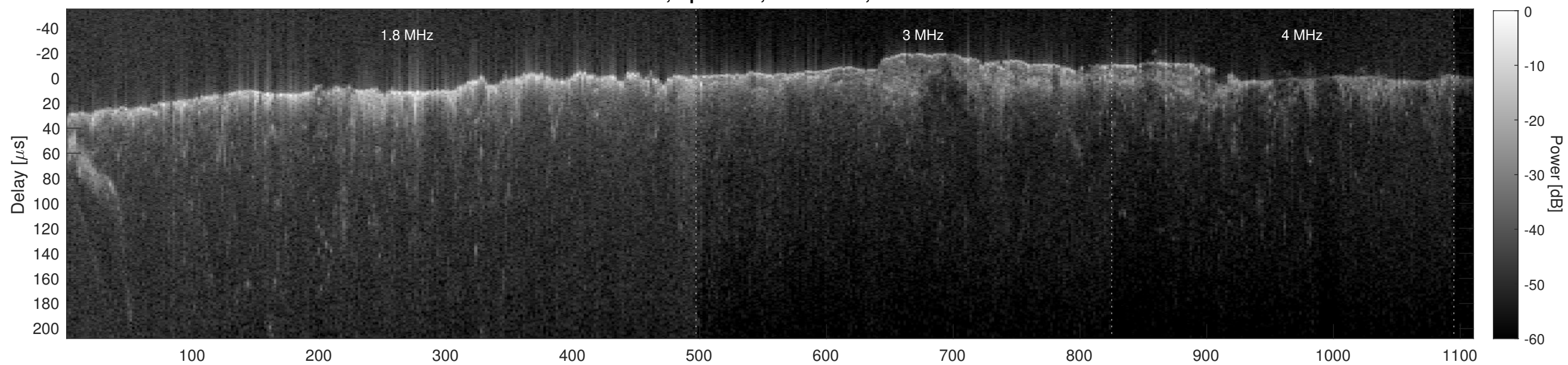
Orbit 2656, Cluttergram
