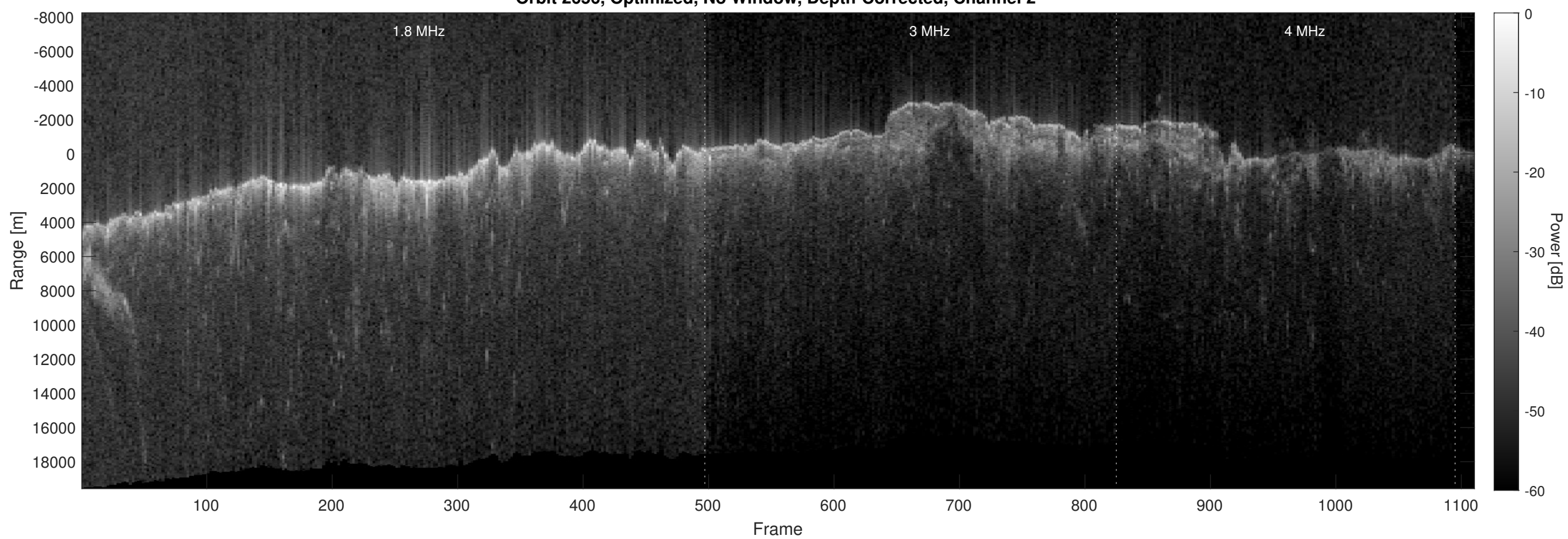
Orbit 2656, Optimized, No Window, Depth-Corrected, Channel 2
