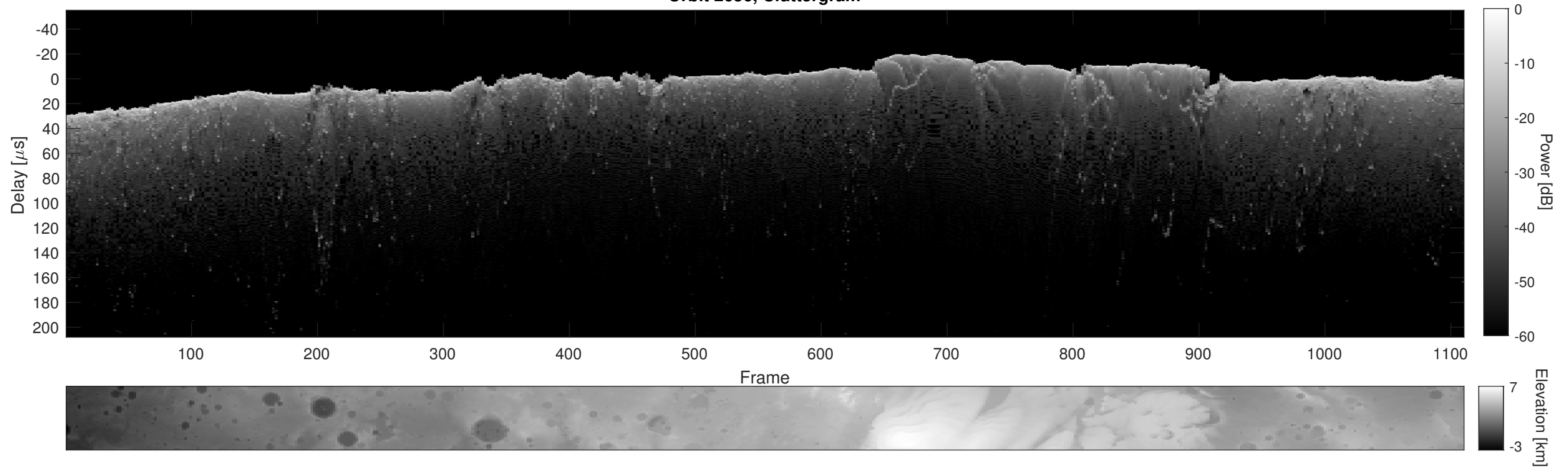
Orbit 2656, Cluttergram
