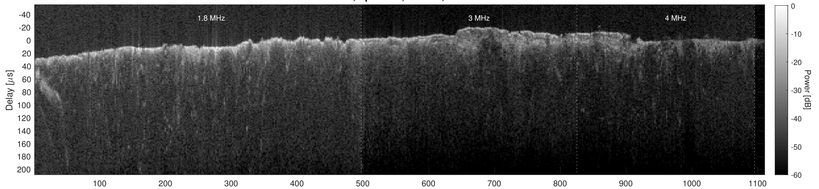
Orbit 2656, Cluttergram
