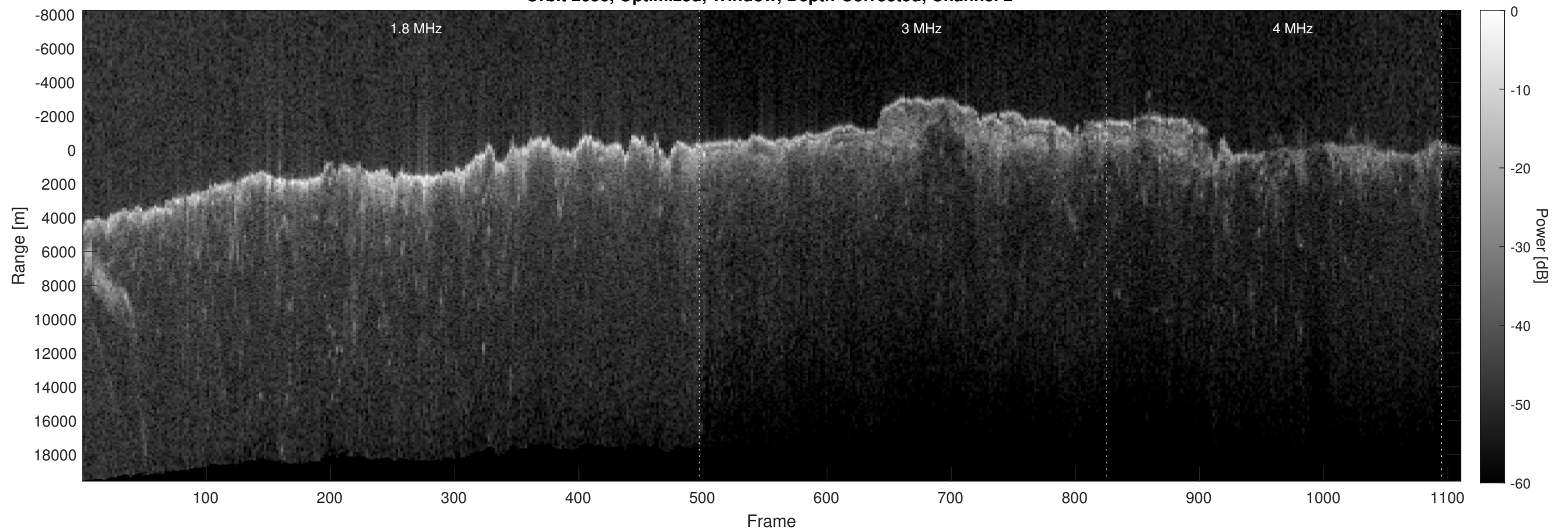
Orbit 2656, Optimized, Window, Depth-Corrected, Channel 2
