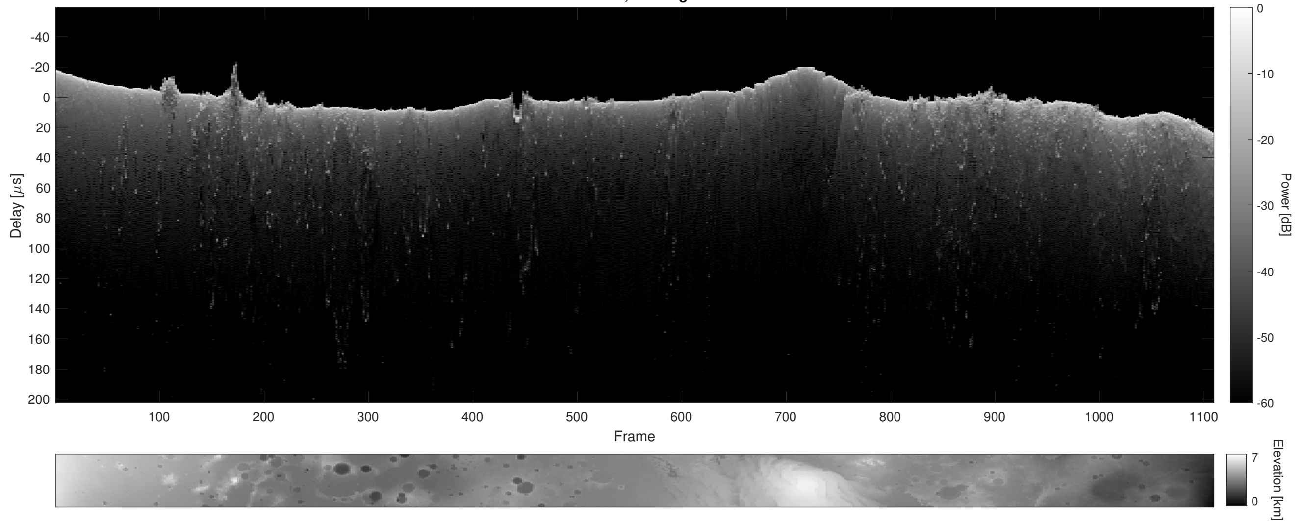
Orbit 2657, Cluttergram
