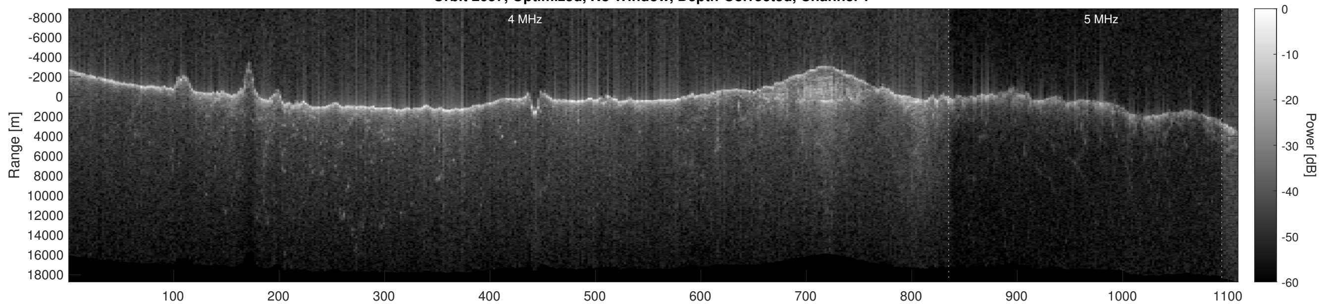
Orbit 2657, Optimized, No Window, Depth-Corrected, Channel 2
