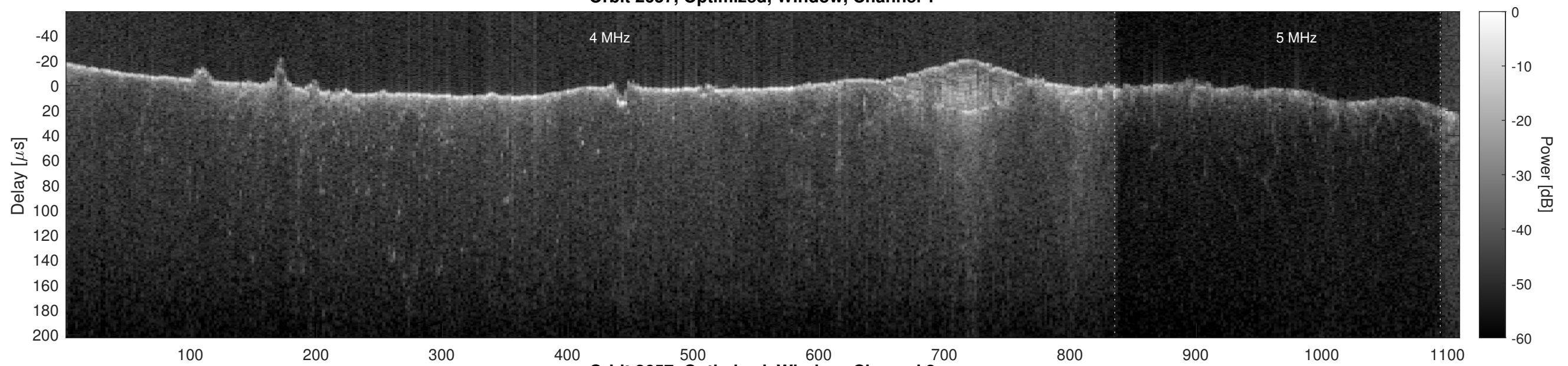
Orbit 2657, Optimized, Window, Channel 2
