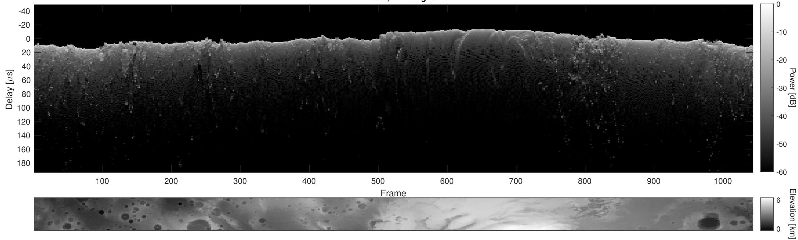
Orbit 2658, Cluttergram
