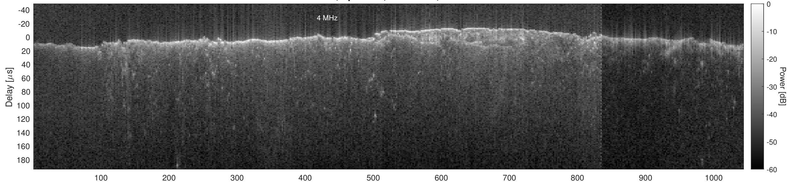
Orbit 2658, Optimized, No Window, Channel 2
