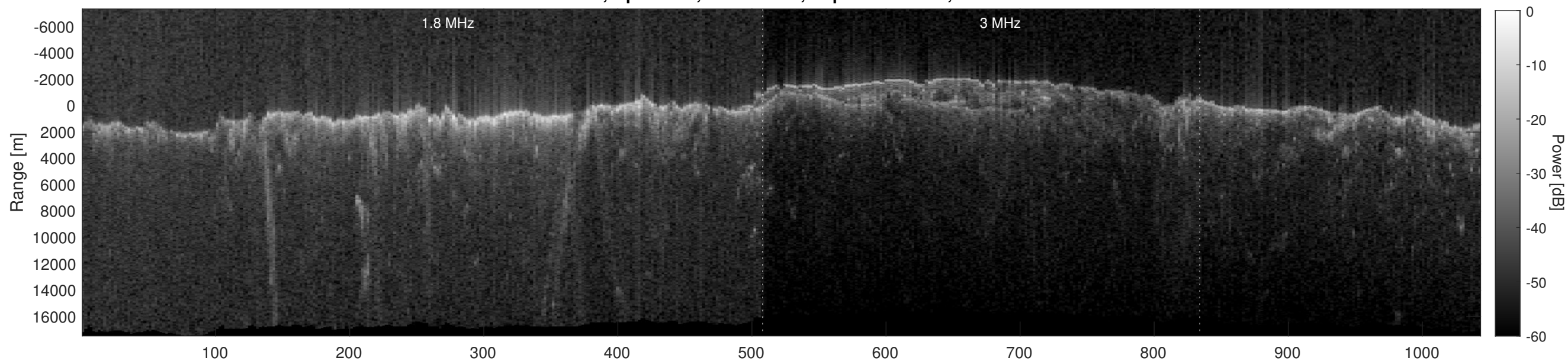
Orbit 2658, Depth-Corrected Cluttergram
