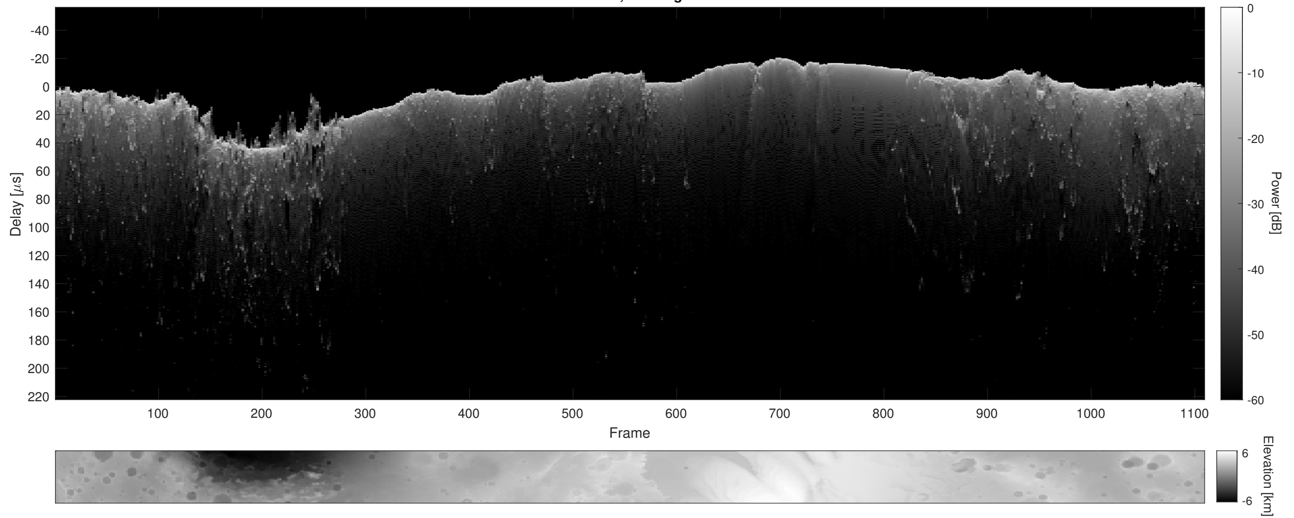
Orbit 2659, Cluttergram
