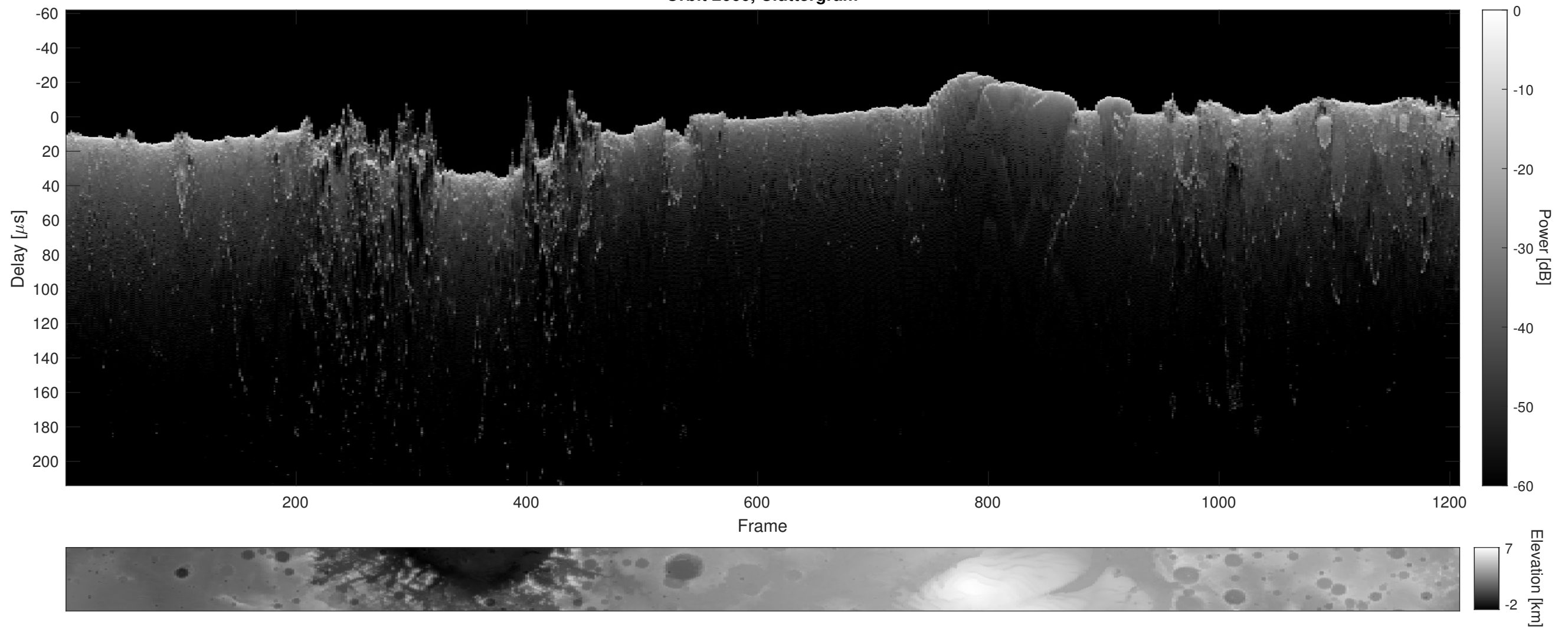
Orbit 2660, Cluttergram
