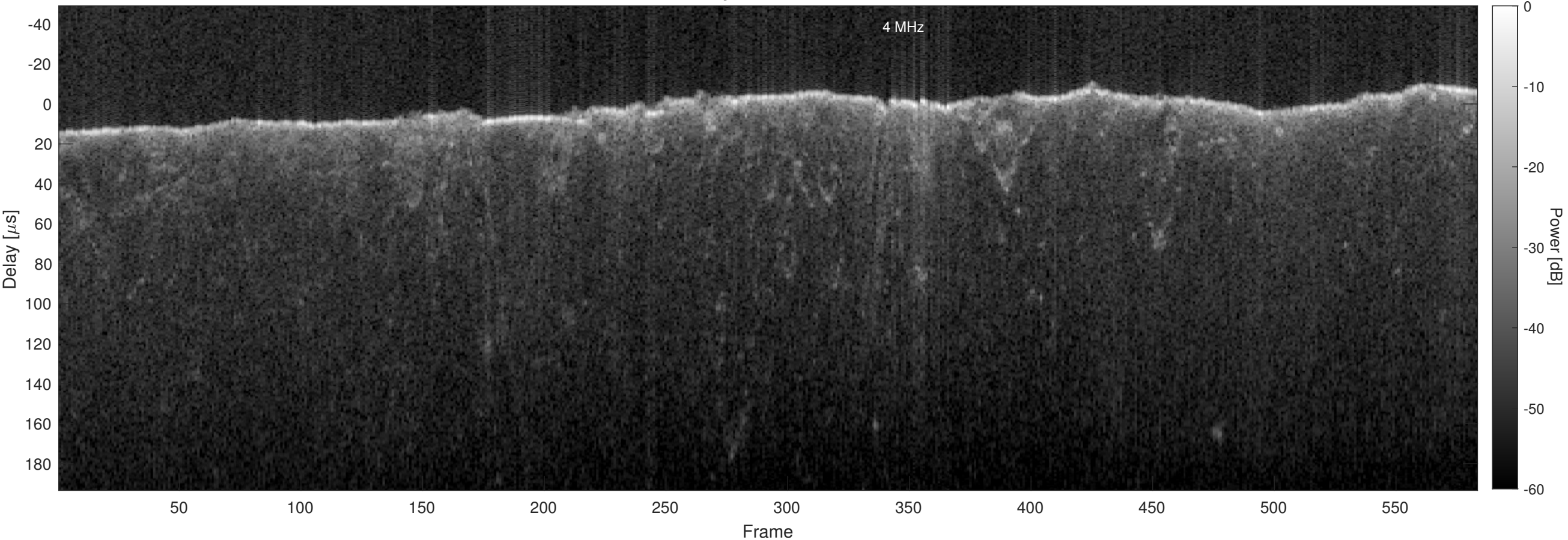
Orbit 2661, Chapman, Window, Channel 2
