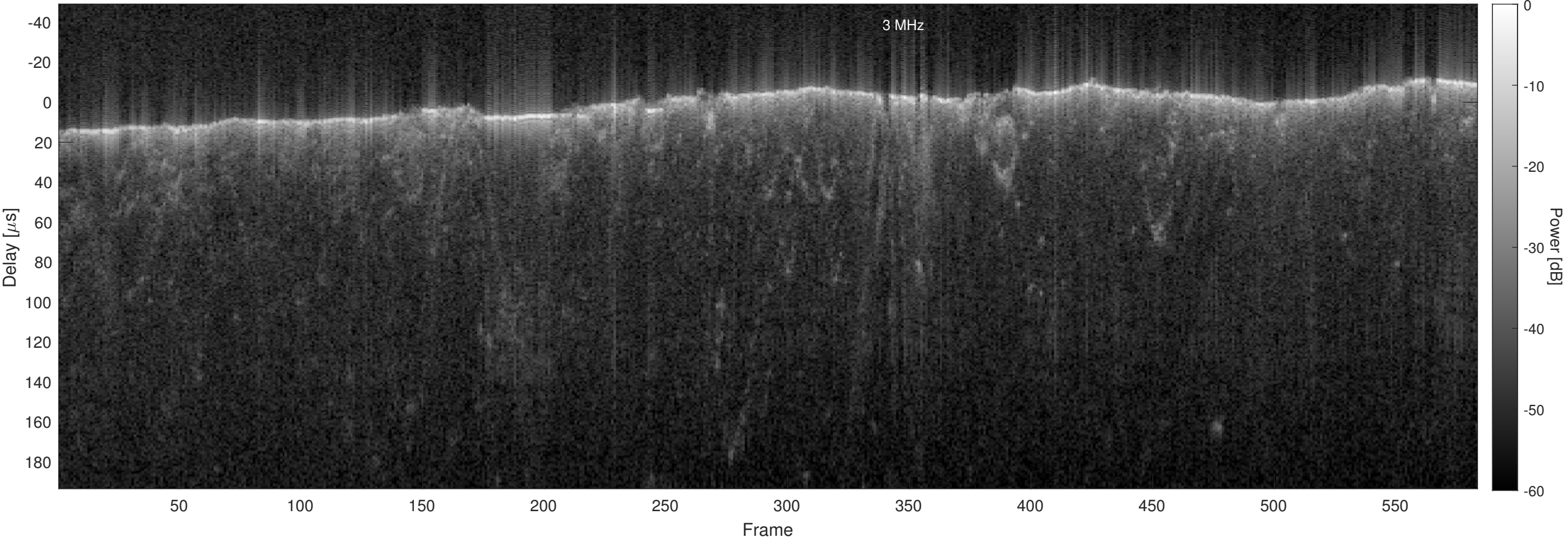
Orbit 2661, Optimized, No Window, Channel 2
