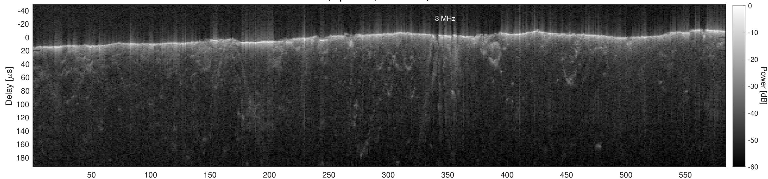
Orbit 2661, Cluttergram
