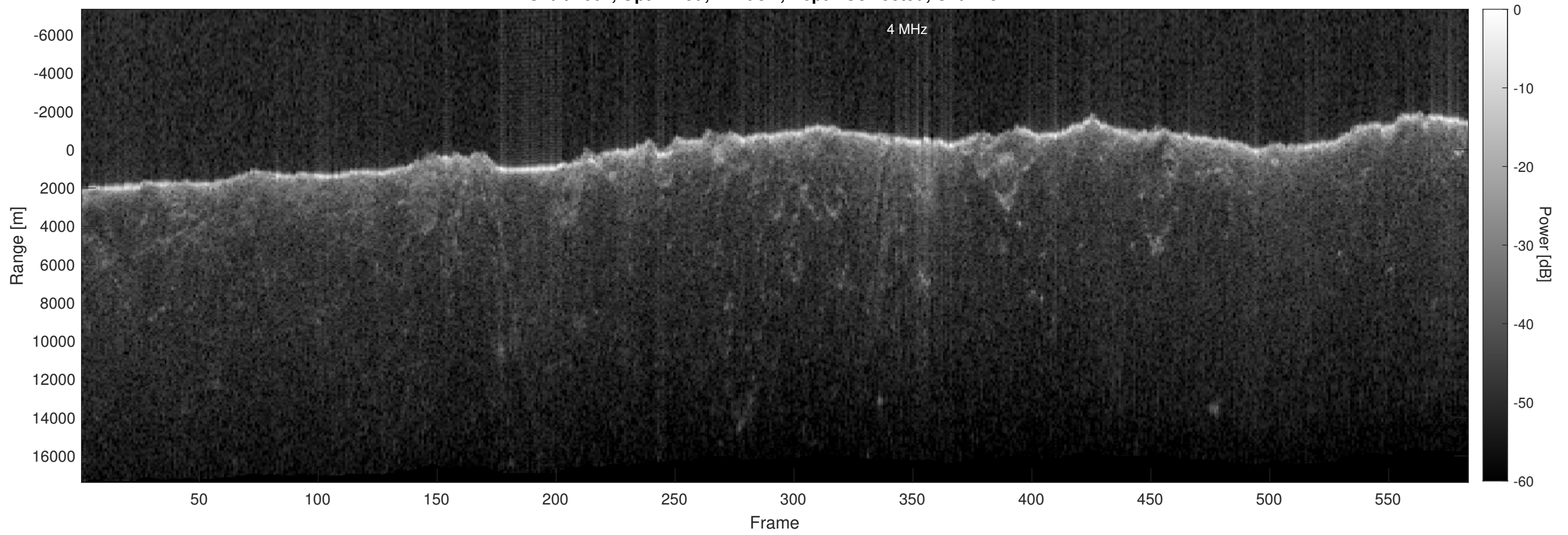
Orbit 2661, Optimized, Window, Depth-Corrected, Channel 2
