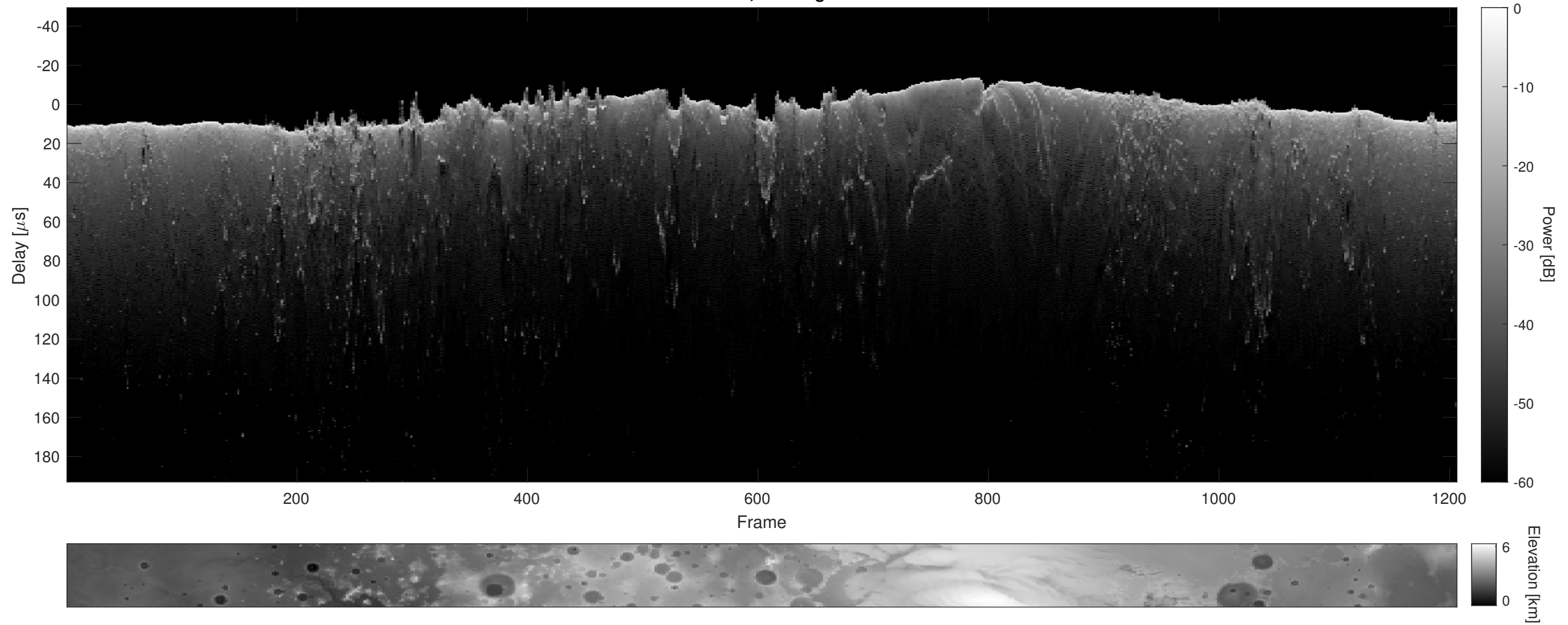
Orbit 2662, Cluttergram
