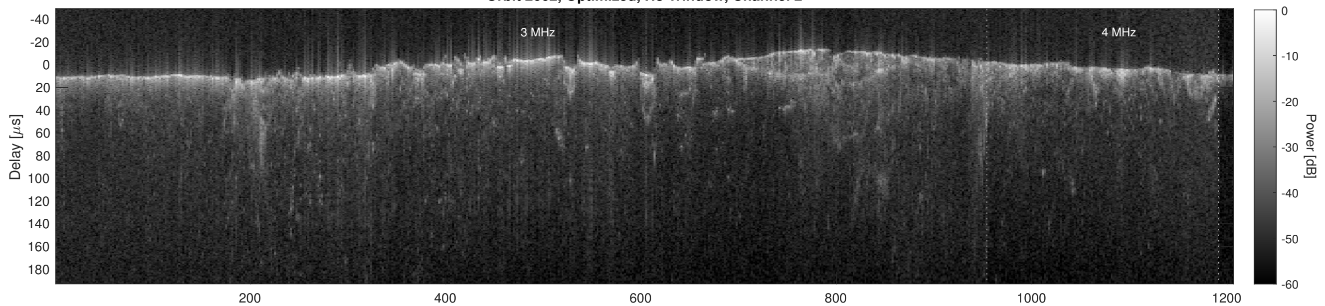
Orbit 2662, Cluttergram
