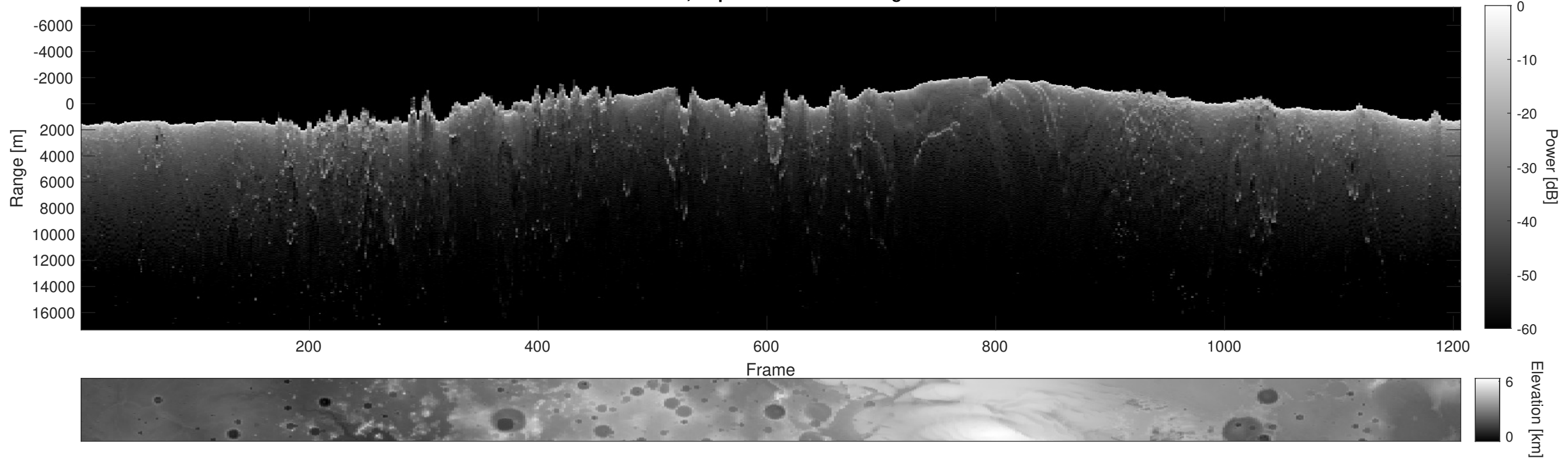
Orbit 2662, Depth-Corrected Cluttergram
