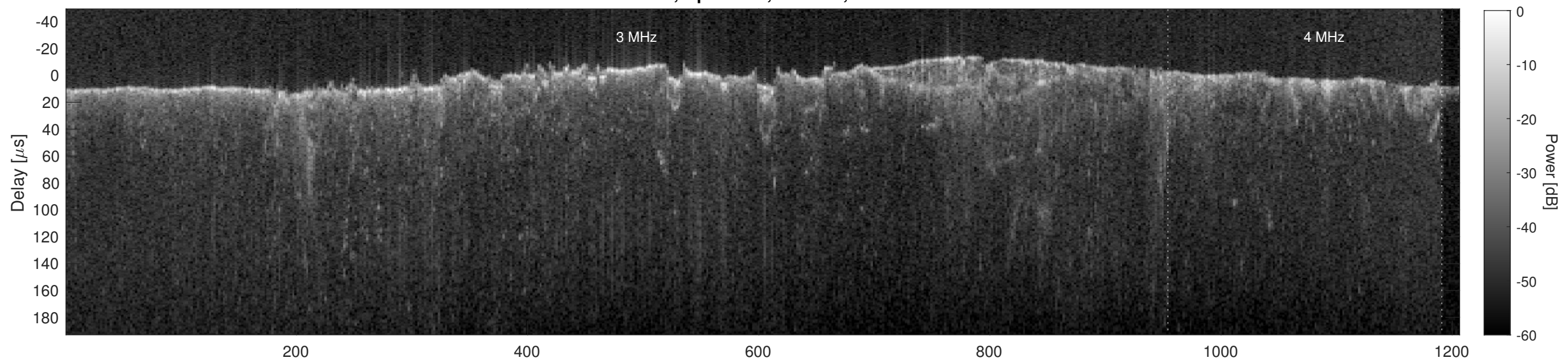
Orbit 2662, Cluttergram
