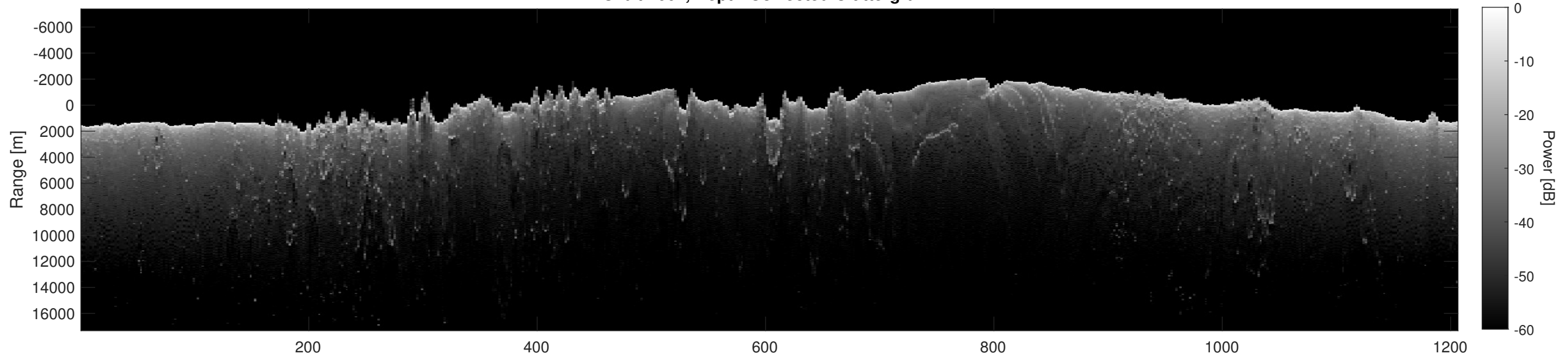
Orbit 2662, Depth-Corrected Cluttergram
