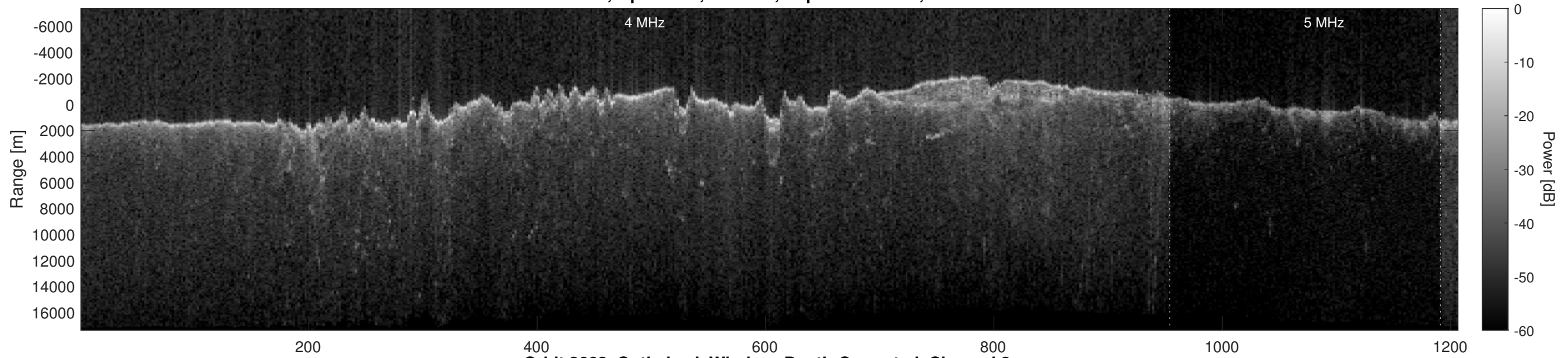
Orbit 2662, Optimized, Window, Depth-Corrected, Channel 2
