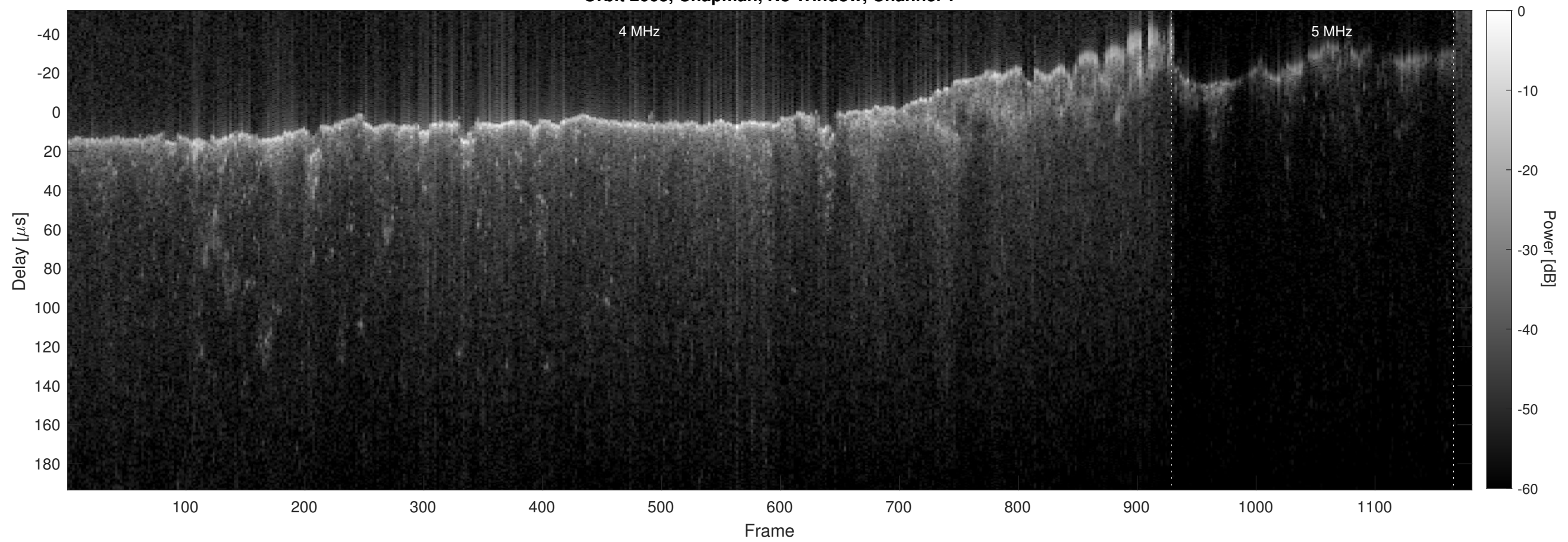
Orbit 2663, Chapman, No Window, Channel 2
