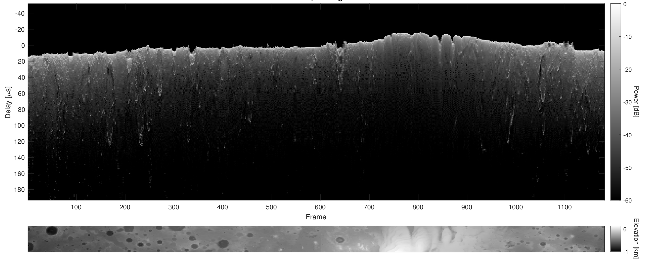
Orbit 2663, Cluttergram
