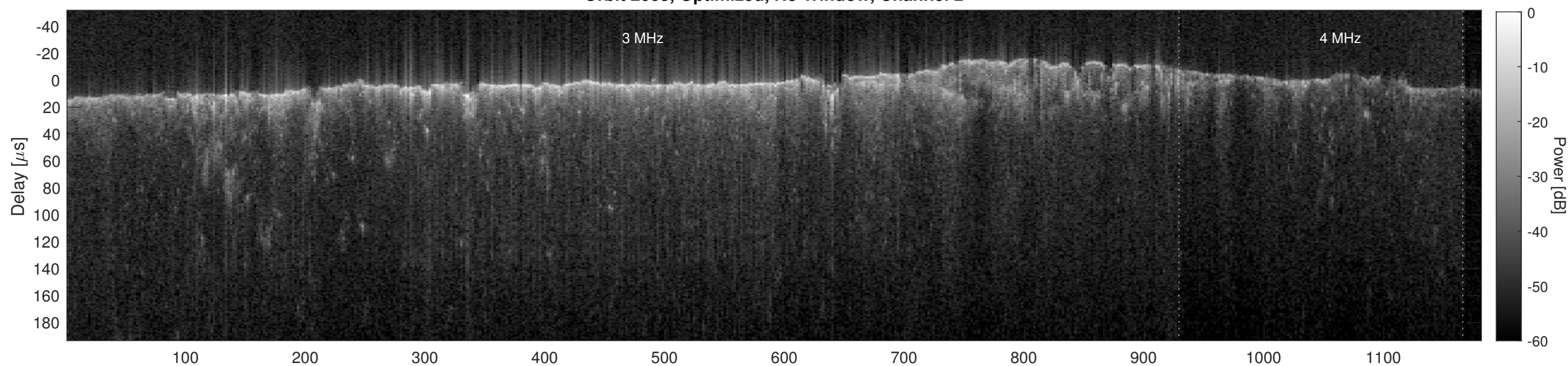
Orbit 2663, Cluttergram
