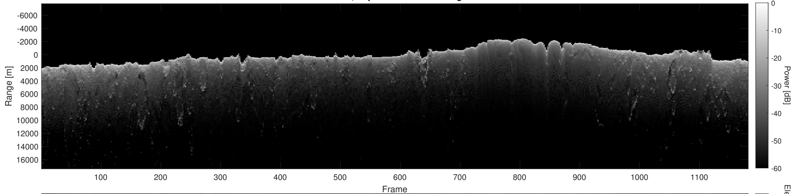
Orbit 2663, Depth-Corrected Cluttergram
