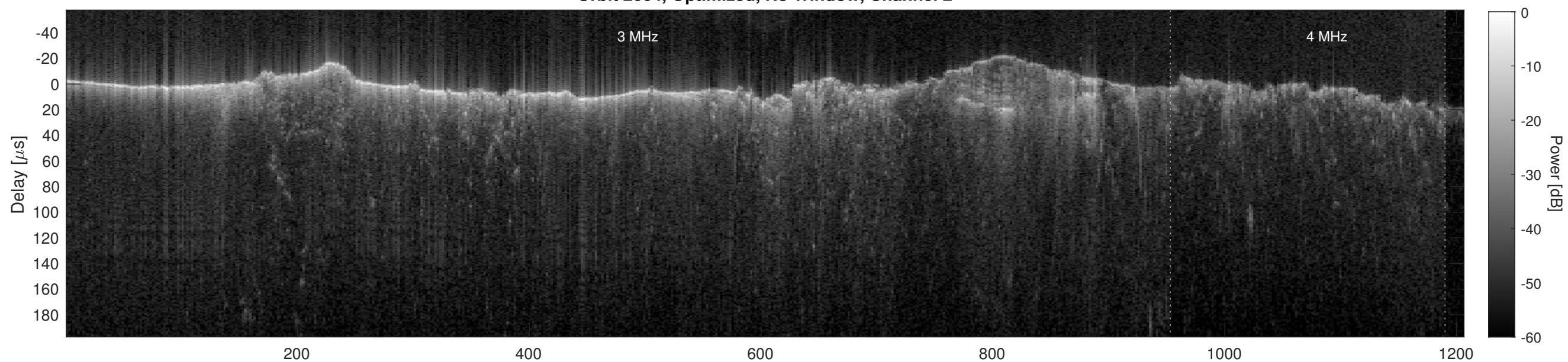
Orbit 2664, Cluttergram
