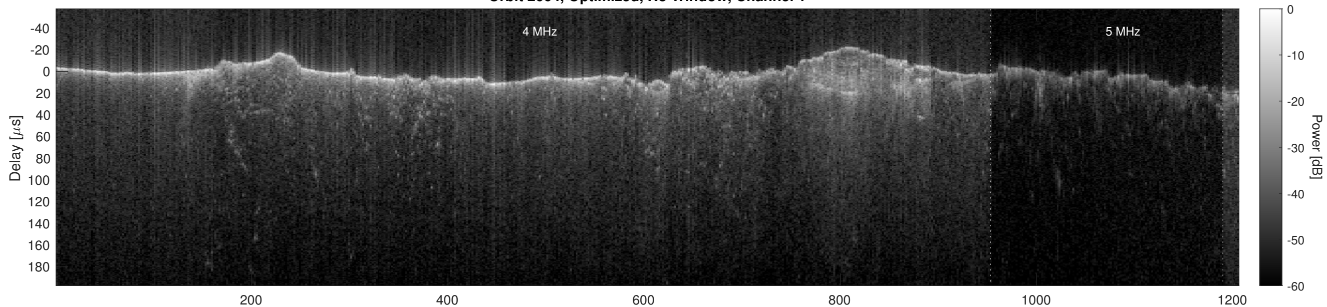
Orbit 2664, Optimized, No Window, Channel 2
