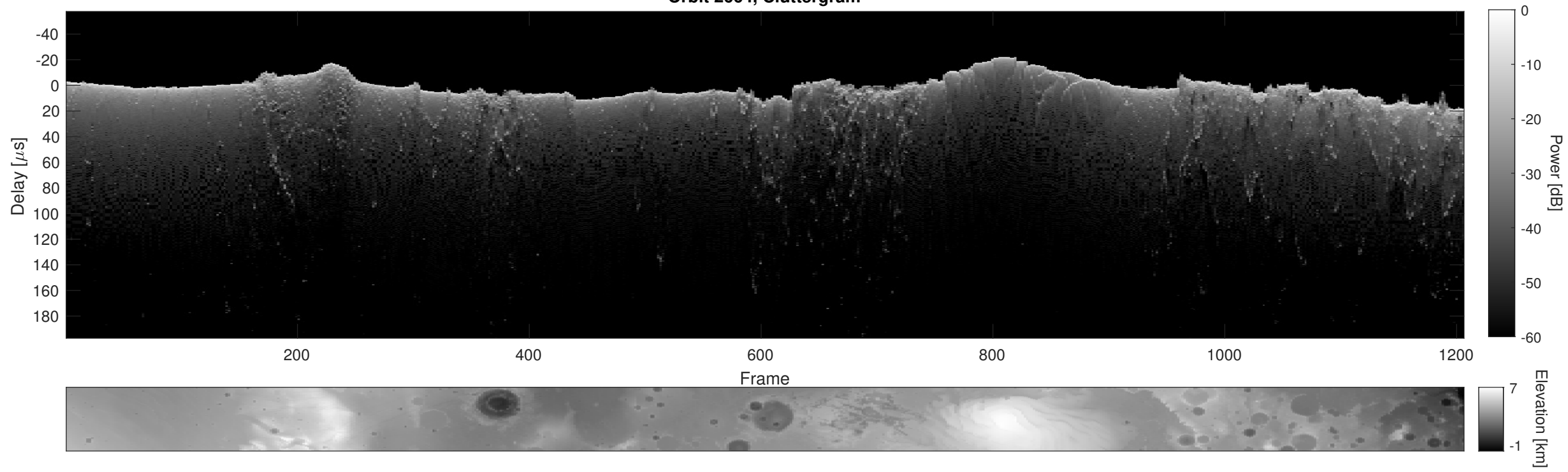
Orbit 2664, Cluttergram
