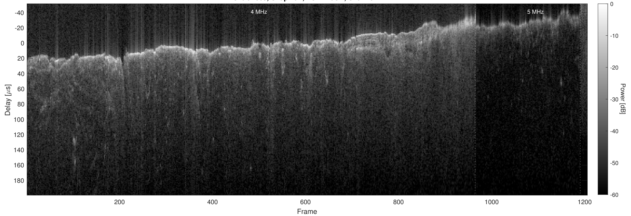
Orbit 2665, Chapman, No Window, Channel 2
