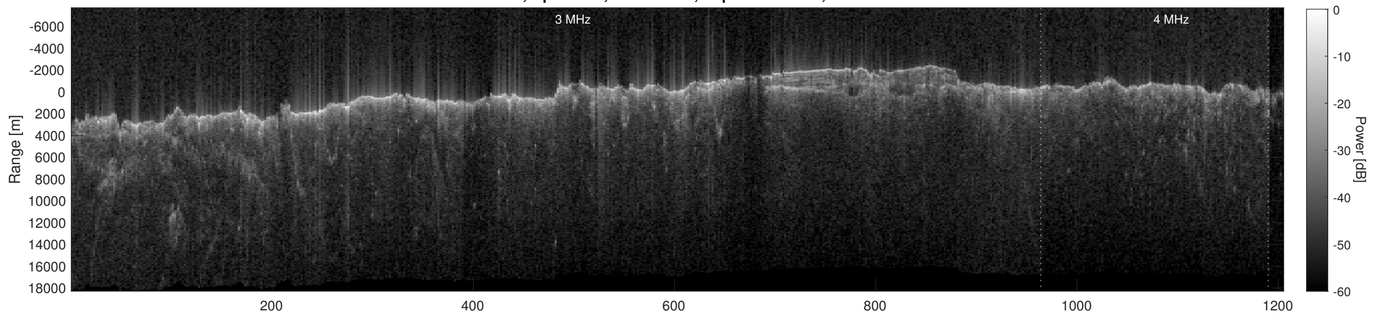
Orbit 2665, Depth-Corrected Cluttergram
