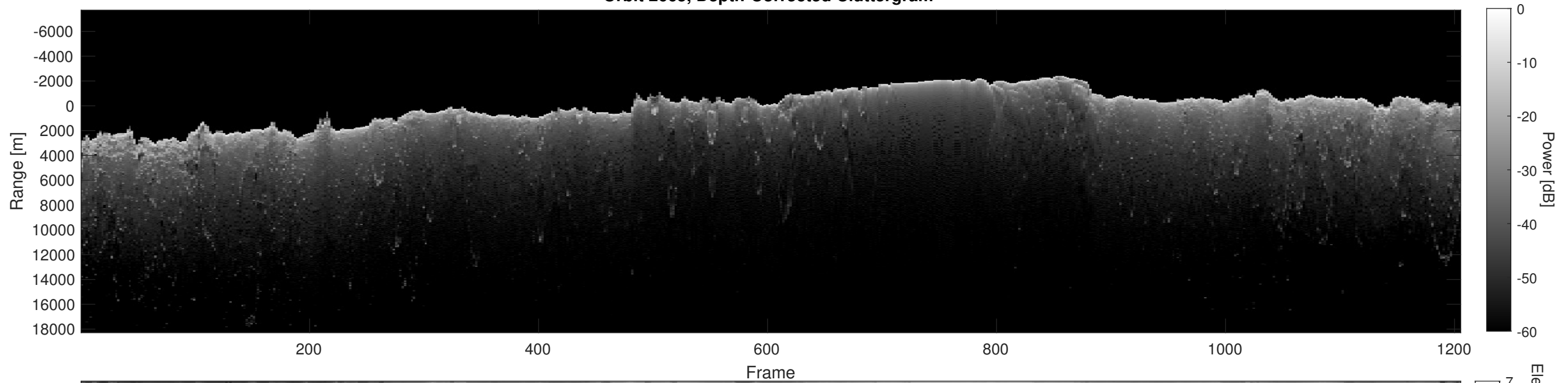
Orbit 2665, Depth-Corrected Cluttergram
