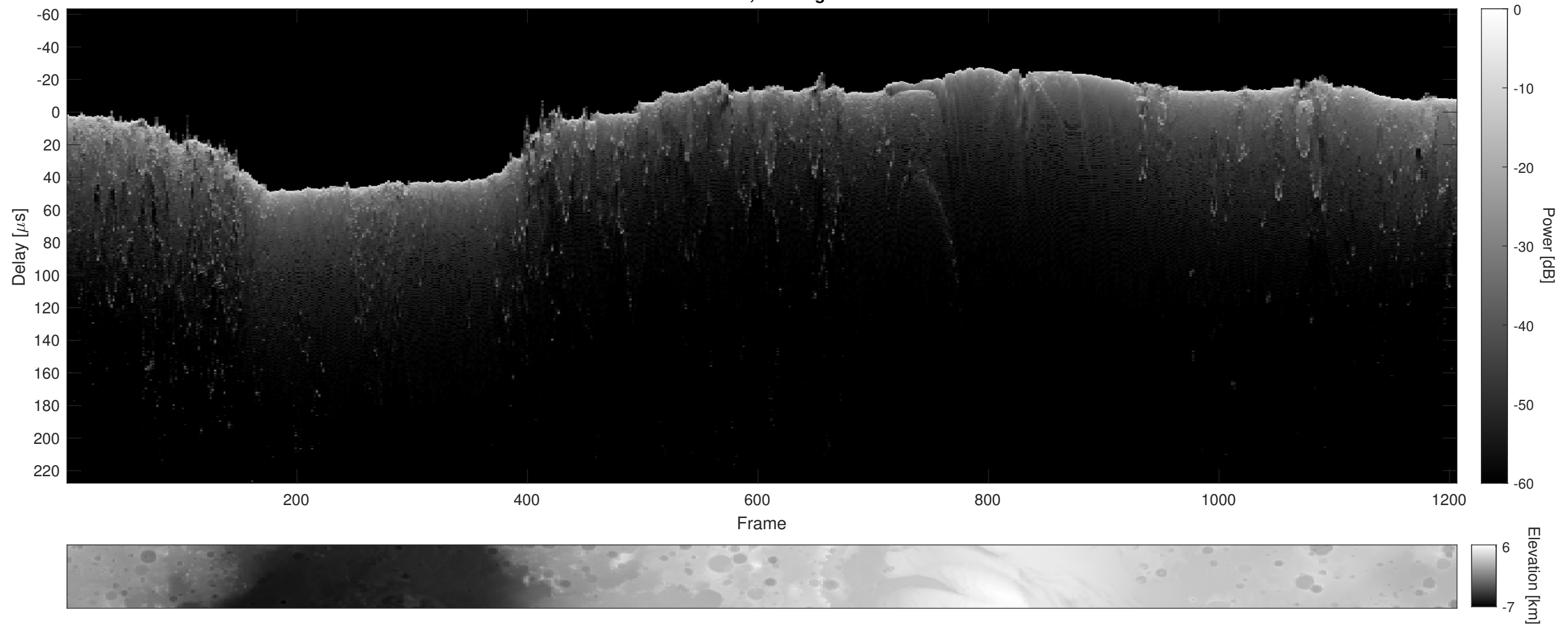
Orbit 2666, Cluttergram
