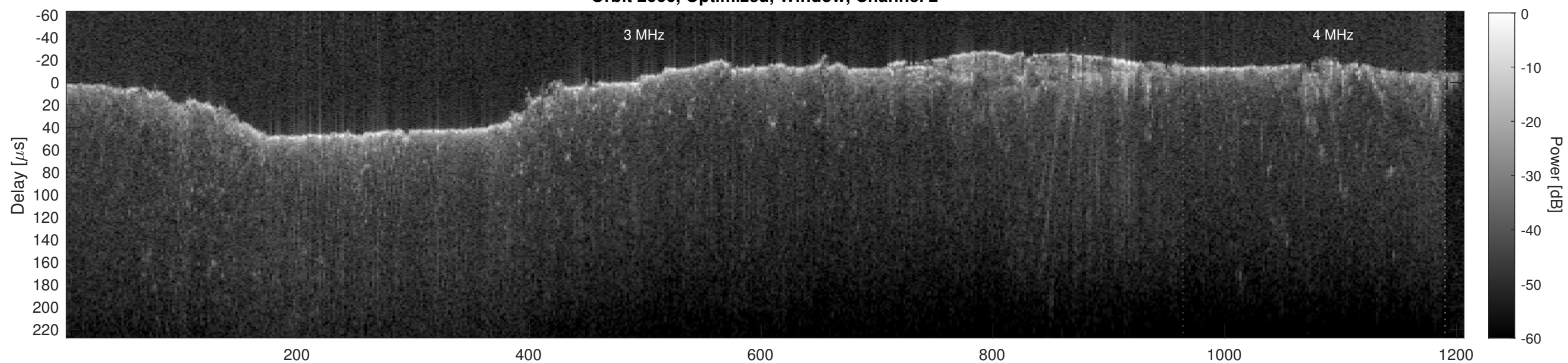
Orbit 2666, Cluttergram
