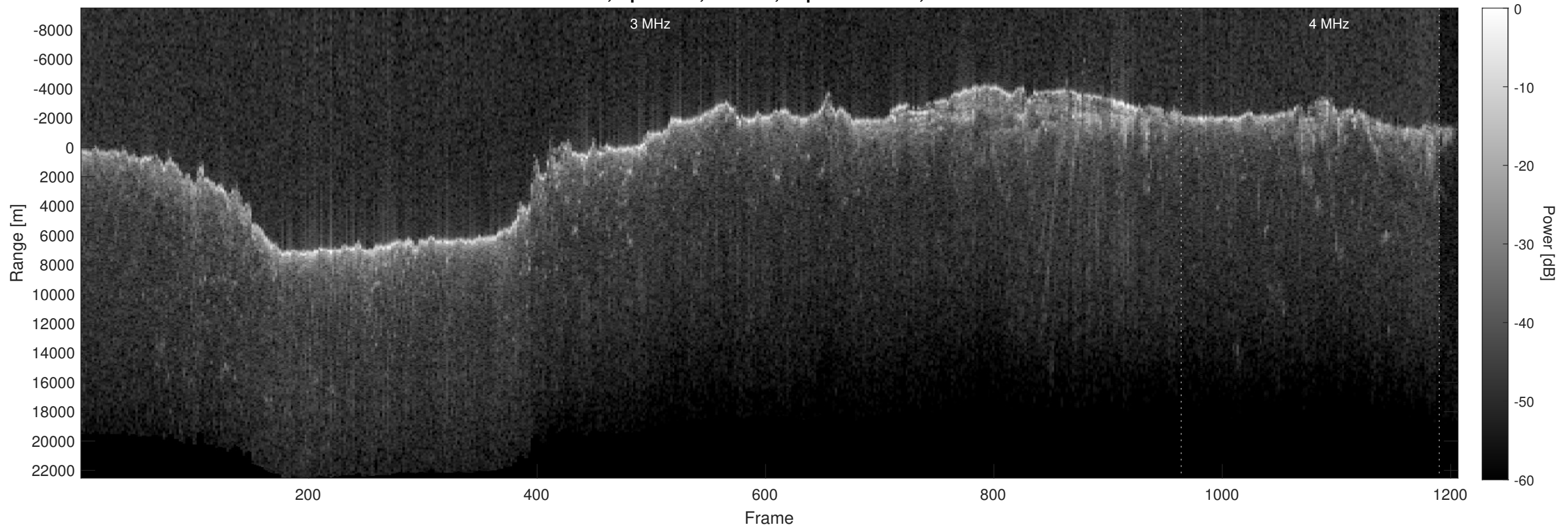
Orbit 2666, Optimized, Window, Depth-Corrected, Channel 2
