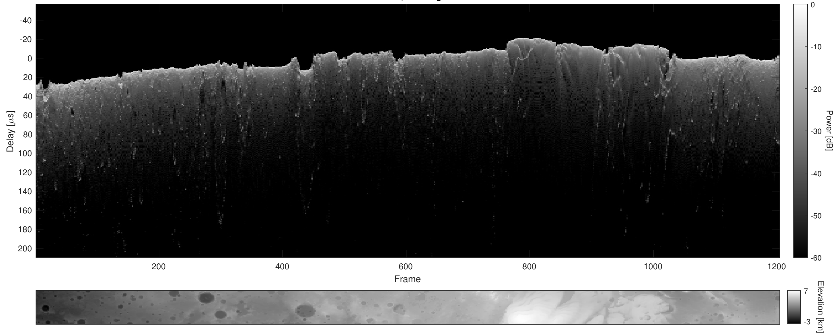
Orbit 2667, Cluttergram
