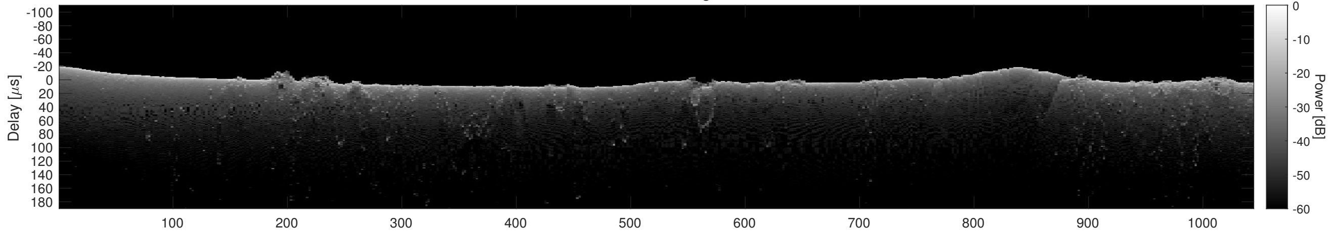
Orbit 2668, Cluttergram
