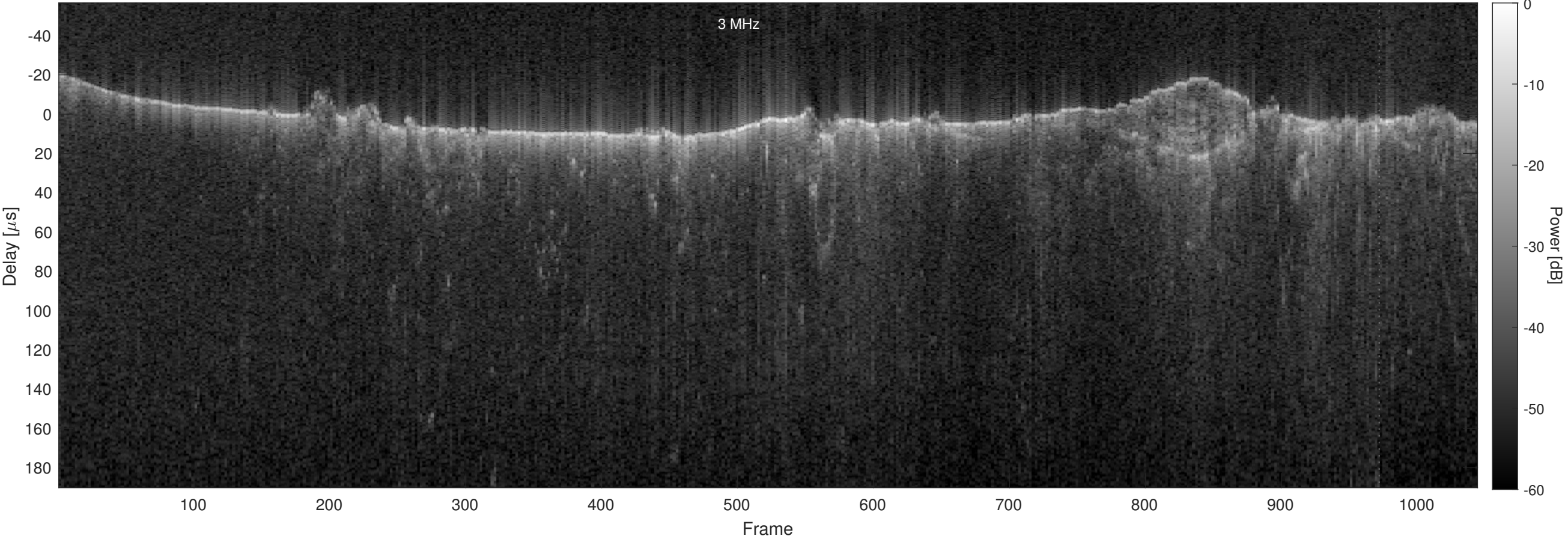
Orbit 2668, Optimized, No Window, Channel 2
