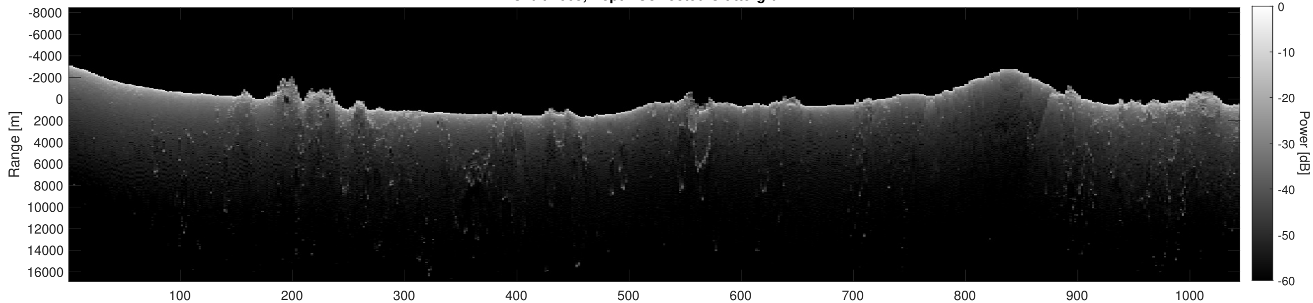
Orbit 2668, Depth-Corrected Cluttergram
