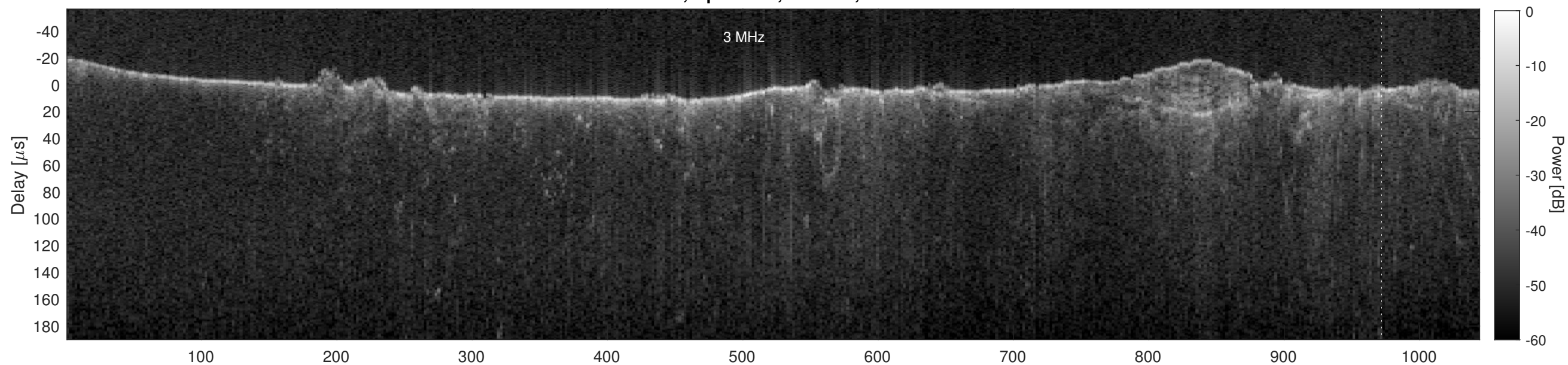
Orbit 2668, Cluttergram
