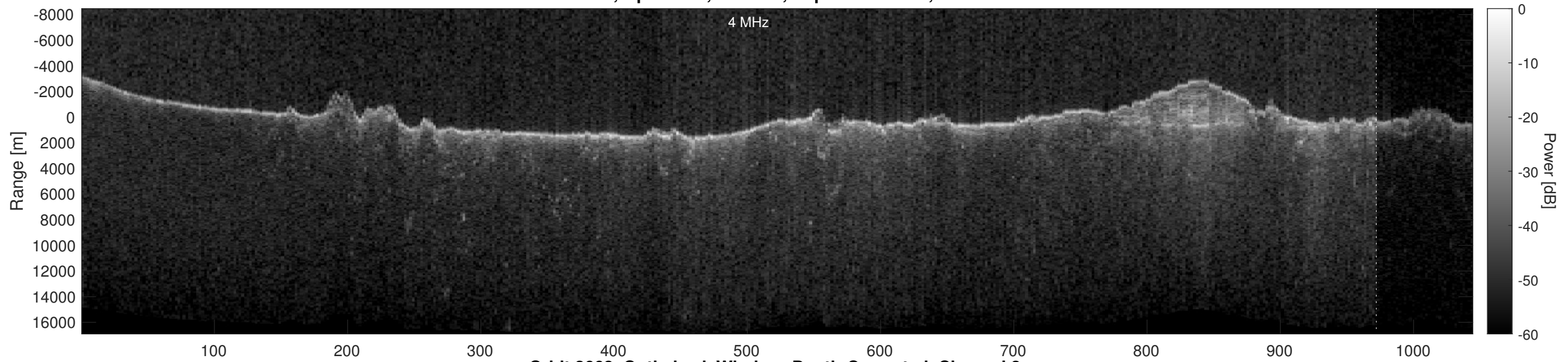
Orbit 2668, Optimized, Window, Depth-Corrected, Channel 2
