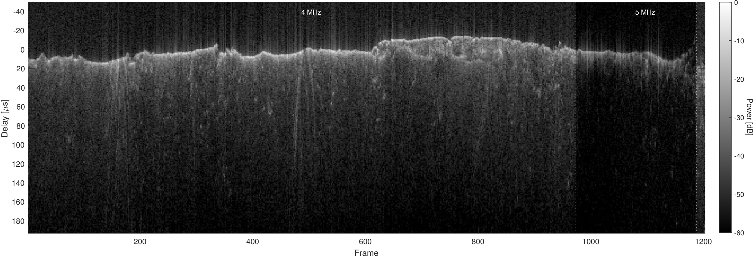
Orbit 2669, Optimized, No Window, Channel 2
