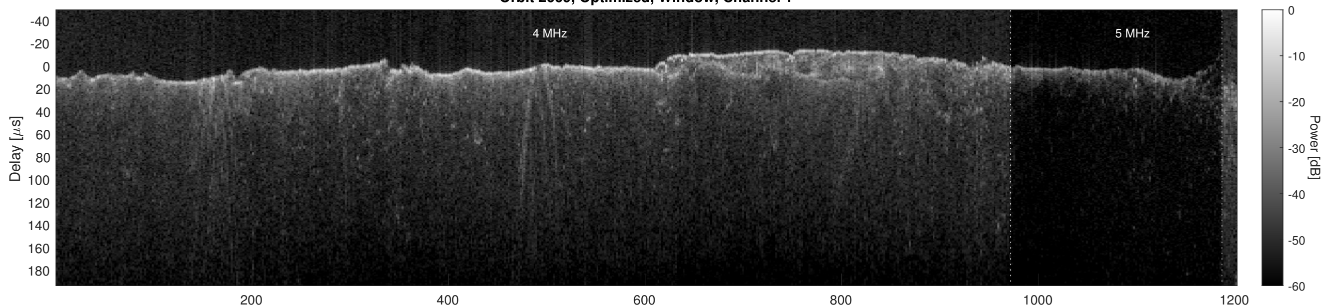
Orbit 2669, Optimized, Window, Channel 2
