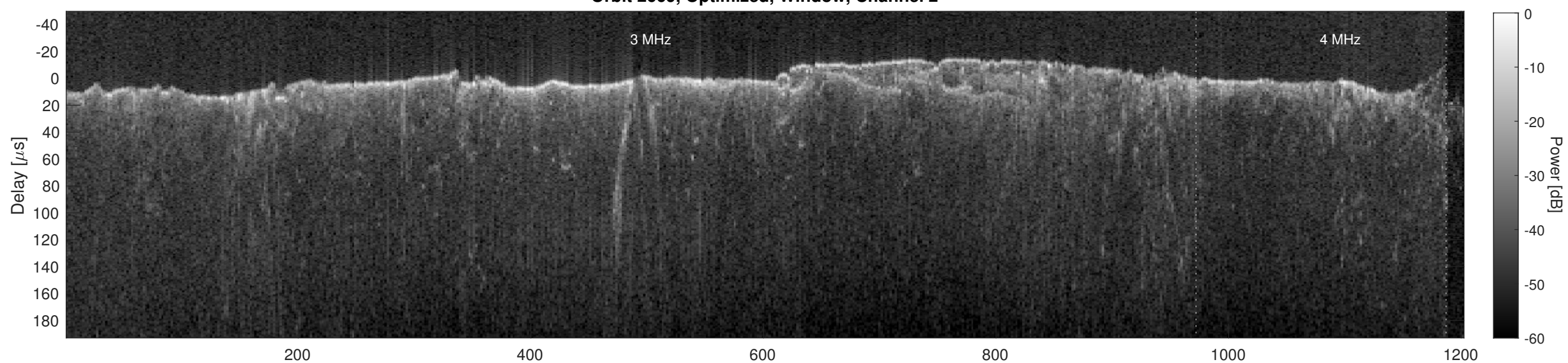
Orbit 2669, Cluttergram
