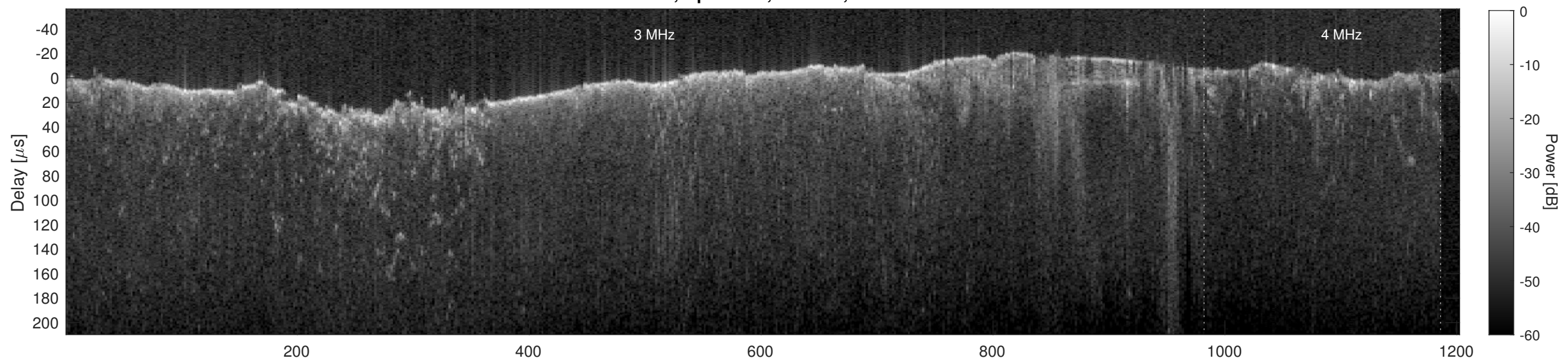
Orbit 2670, Cluttergram
