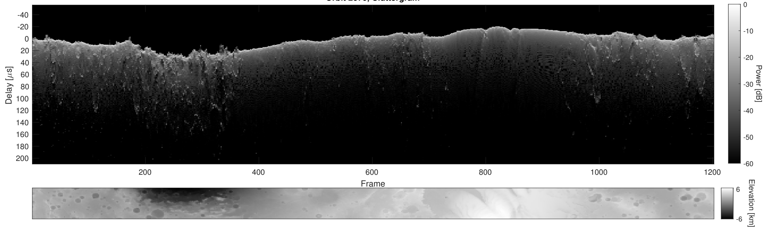
Orbit 2670, Cluttergram
