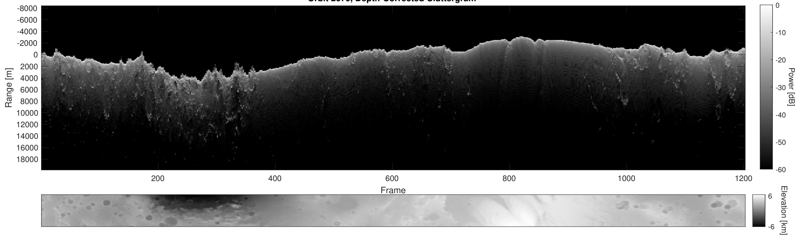
Orbit 2670, Depth-Corrected Cluttergram
