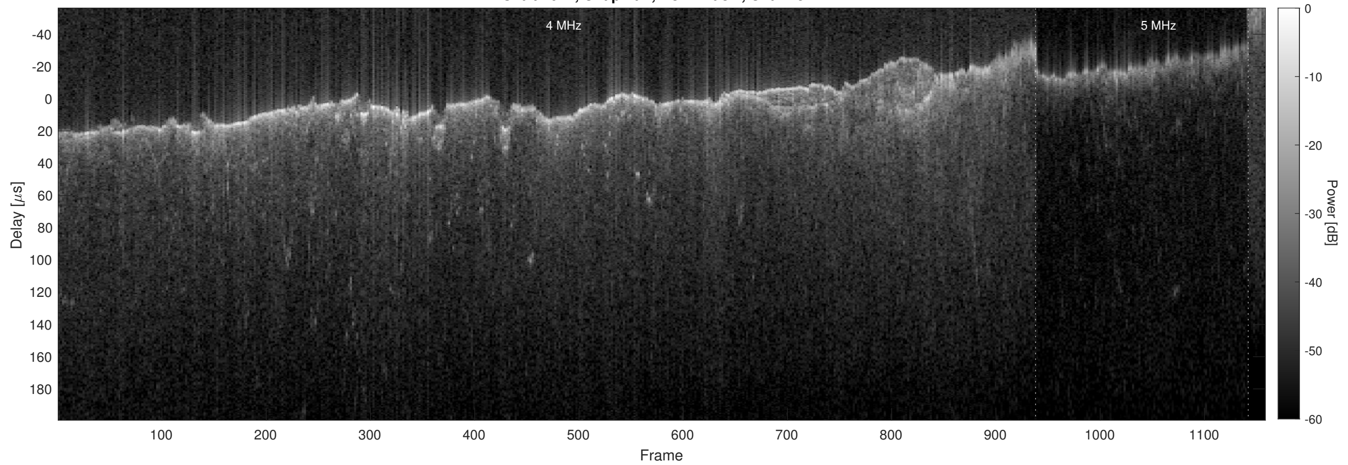
Orbit 2672, Chapman, No Window, Channel 2
