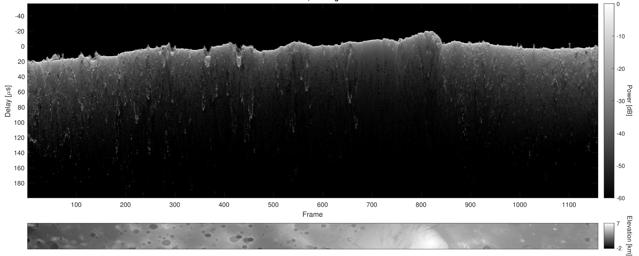
Orbit 2672, Cluttergram
