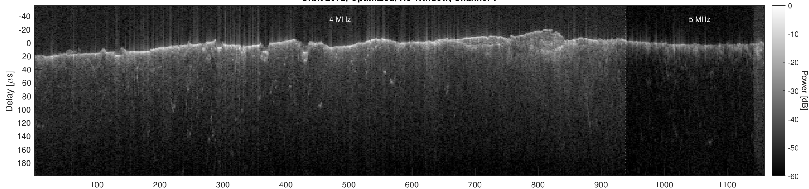
Orbit 2672, Optimized, No Window, Channel 2
