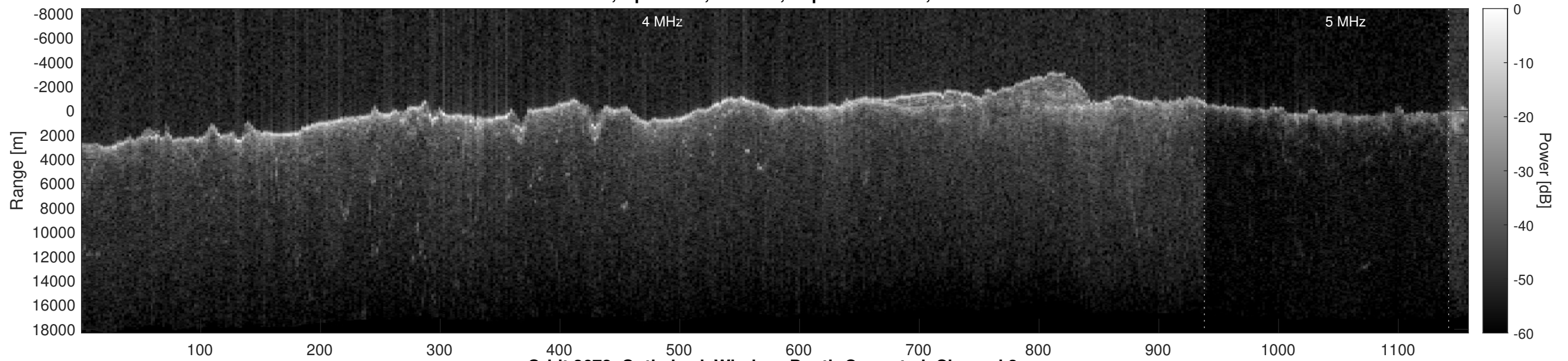
Orbit 2672, Optimized, Window, Depth-Corrected, Channel 2
