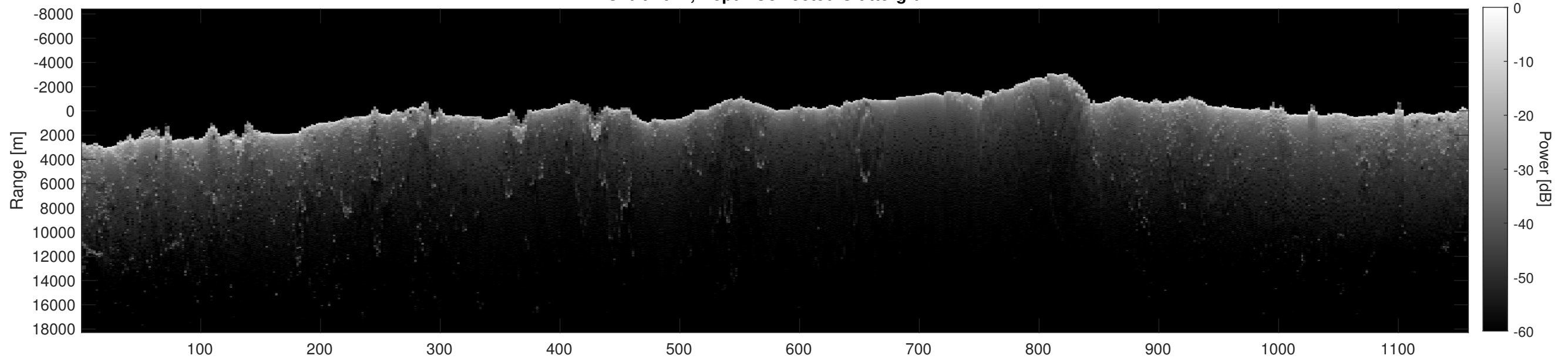
Orbit 2672, Depth-Corrected Cluttergram
