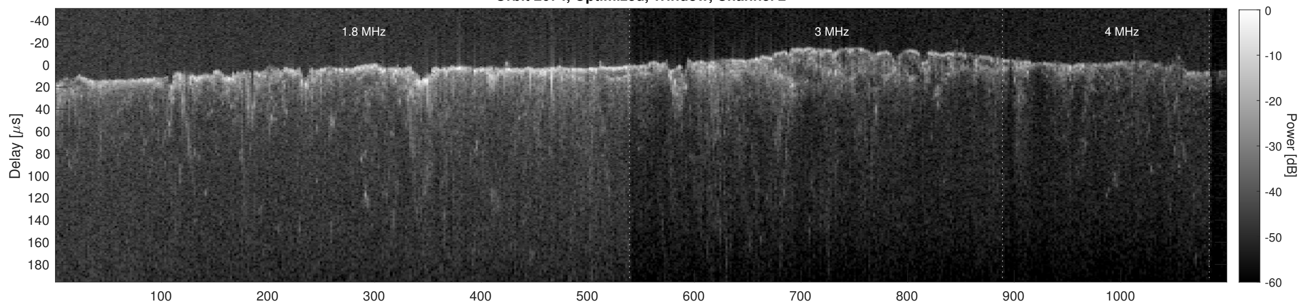
Orbit 2674, Cluttergram
