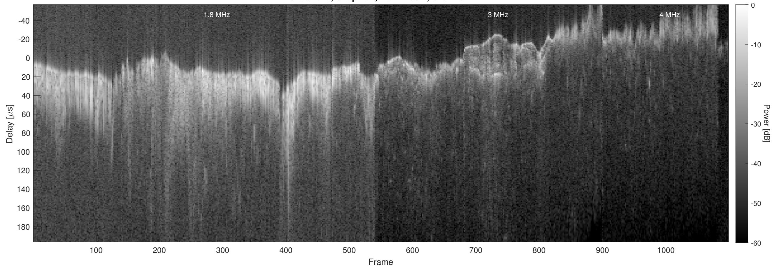
Orbit 2675, Chapman, No Window, Channel 2
