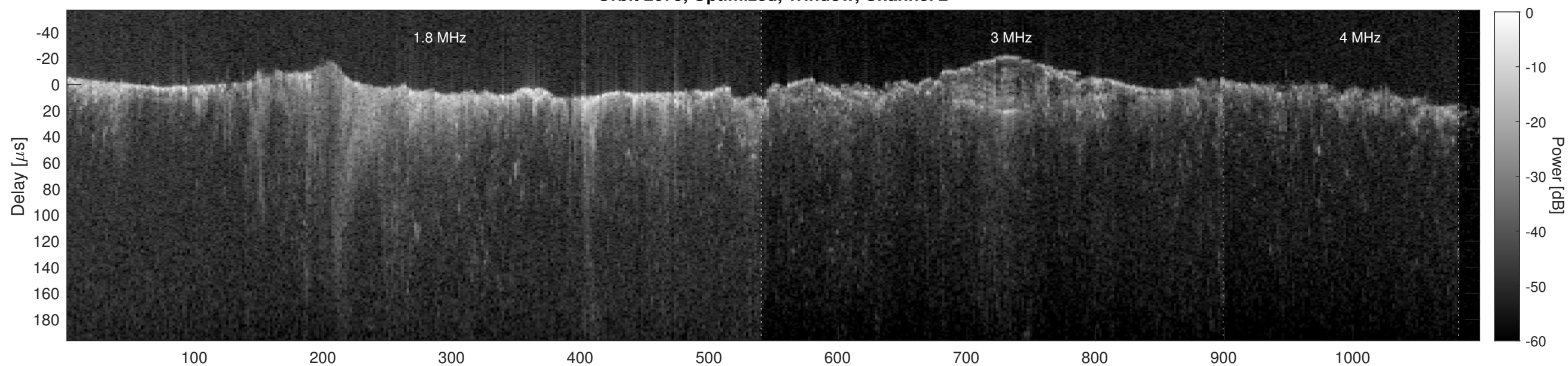
Orbit 2675, Cluttergram
