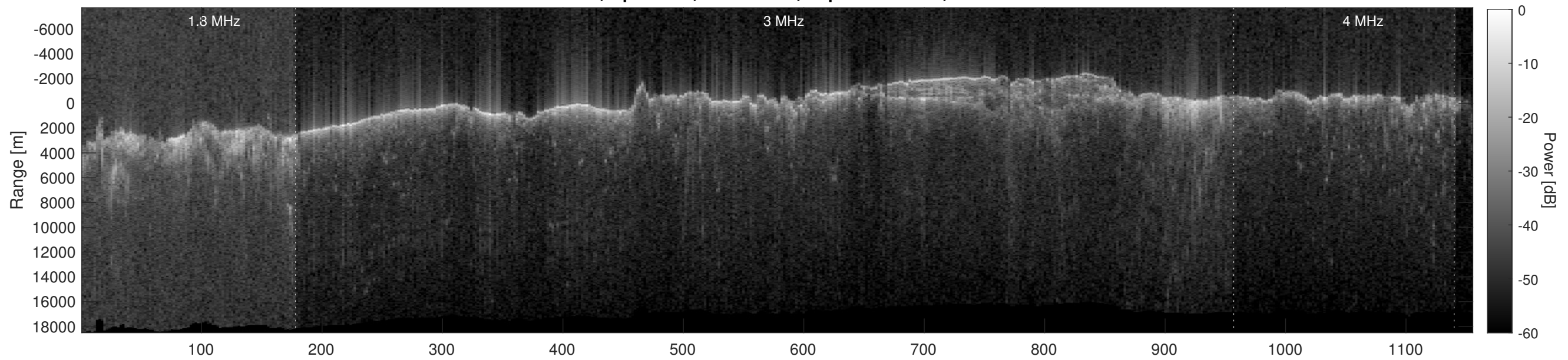
Orbit 2676, Depth-Corrected Cluttergram
