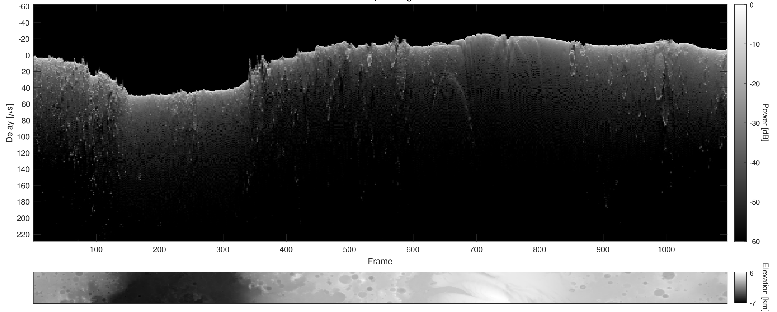
Orbit 2677, Cluttergram
